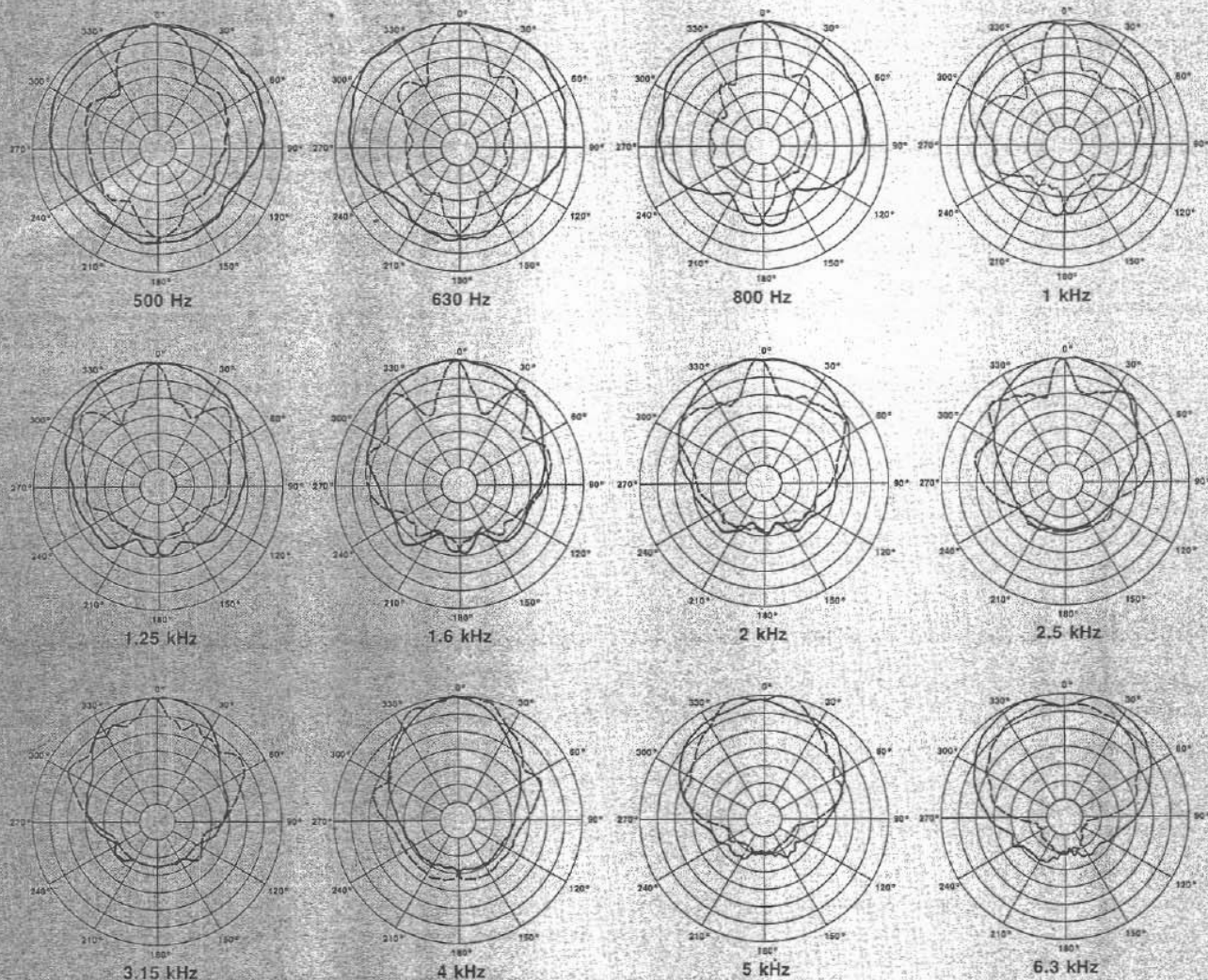
FIGURE 1 LR4B Polar Response
