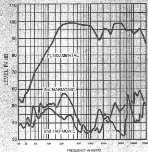
FIGURE 3 LR4B Frequency Response (1 watt at 1 meter)
