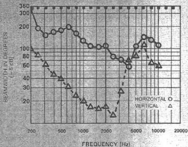
FIGURE 2 LR4B Beamwidth vs. Frequency
